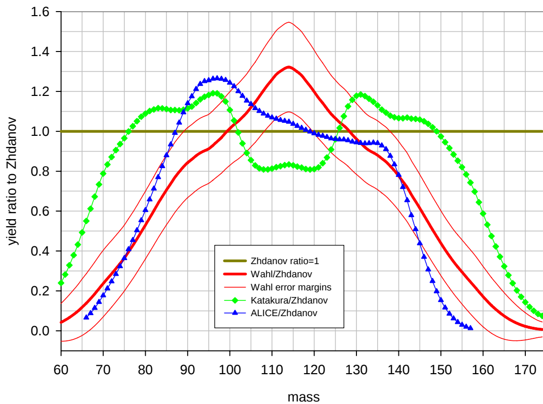
Benchmark B: ^{237}\text{Np} at 100 MeV, post neutron emission yield ratio to Zhdanov's data
